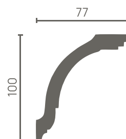
DD08 — 100x77x2000 mm
