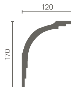
DD511 — 170x120x2000 mm
