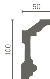
DD503 — 100x50x2000 mm
