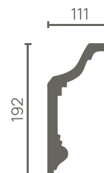
DD513 — 192x111x2000 mm
