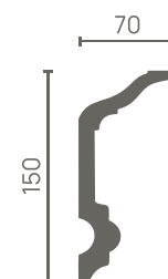
DD505 — 150x70x2000 mm
