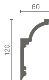
DD517 — 120x60x2000 mm
