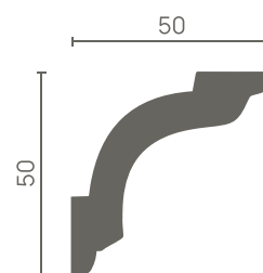
DD42 — 50x50x2000 mm
